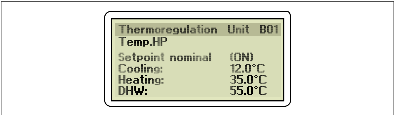
FIG. 73 (Menù Setpoint)
